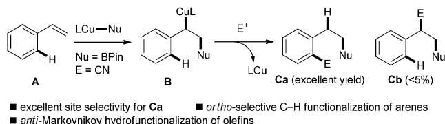
Scheme 1. Copper-catalyzed borylation/ ortho C–H cyanation of styrenes. Pin = pinacol.
